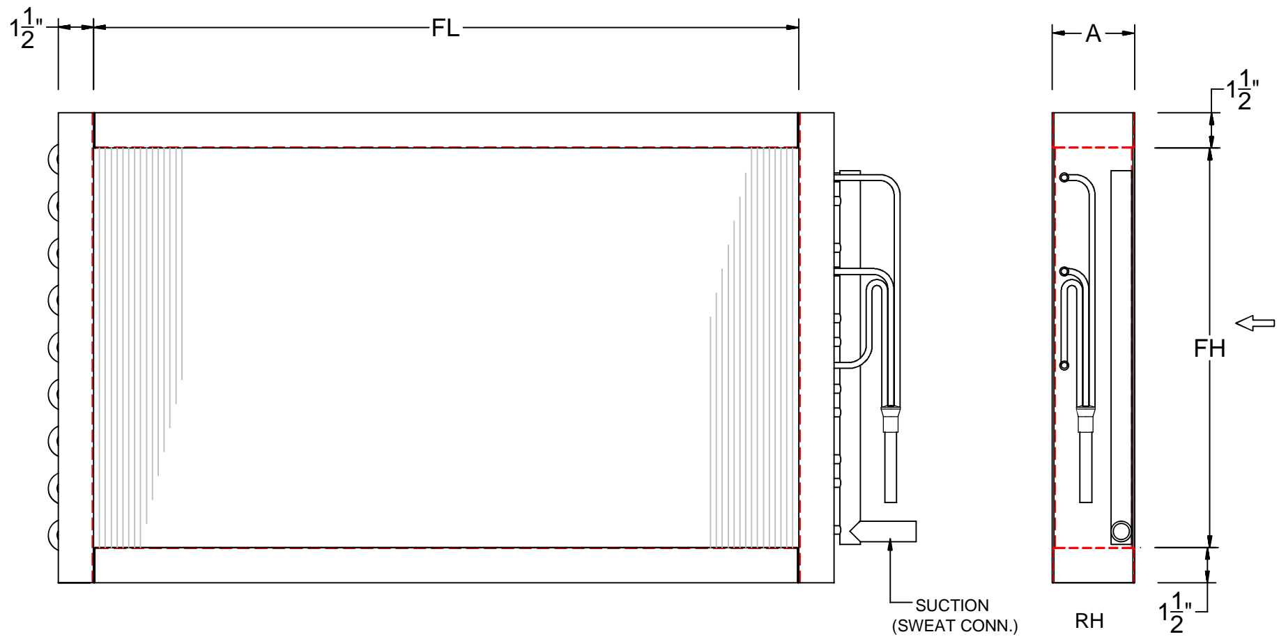
DIRECT EXPANSION EVAPORATOR
