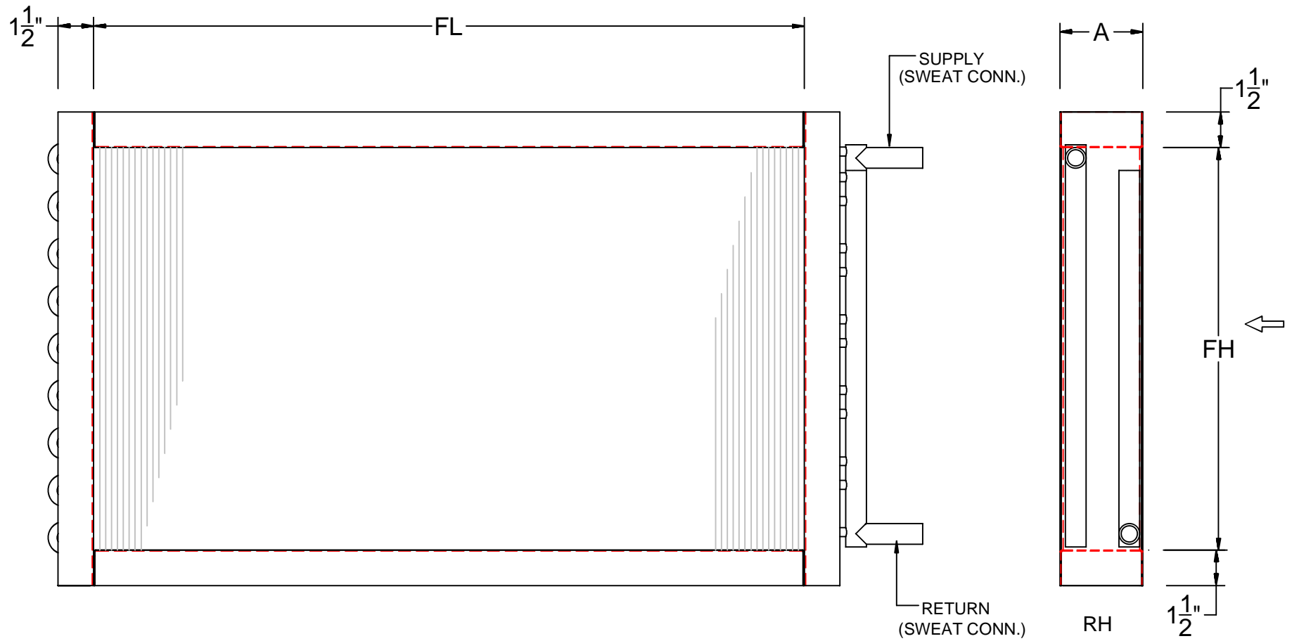
REFRIGERANT CONDENSER AND HEAT RECLAIM
