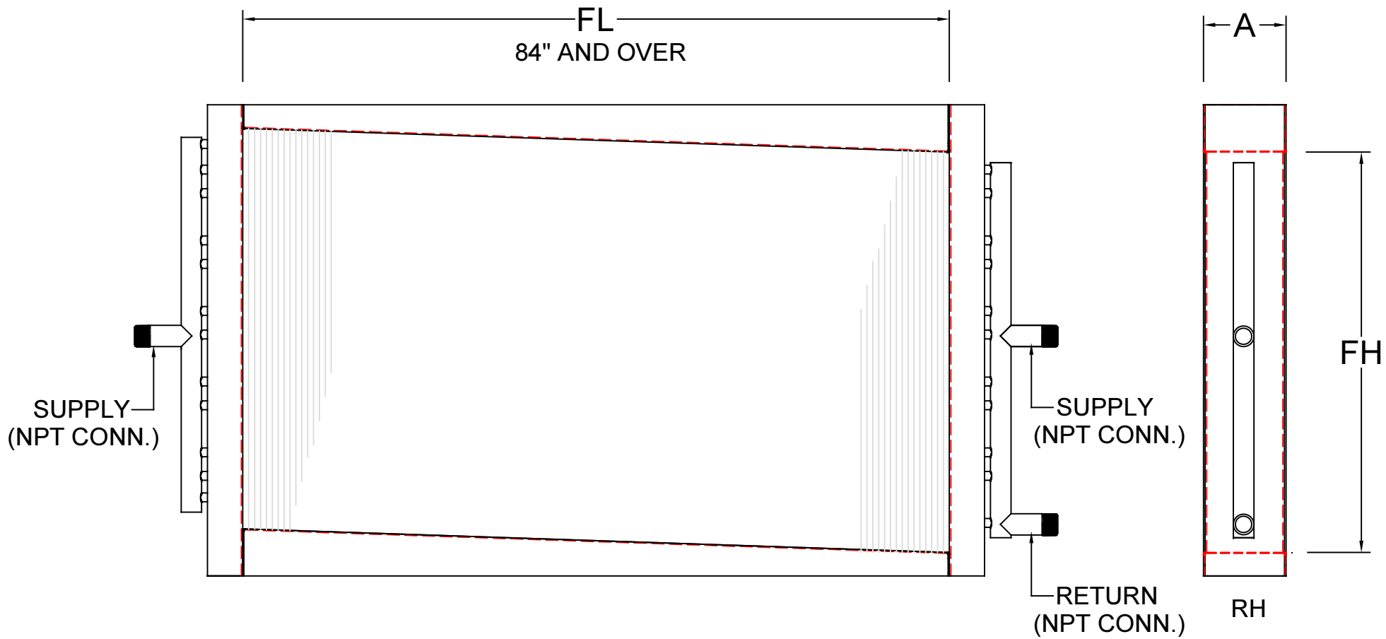
STEAM DISTRIBUTING (WITH TWO SUPPLY)
