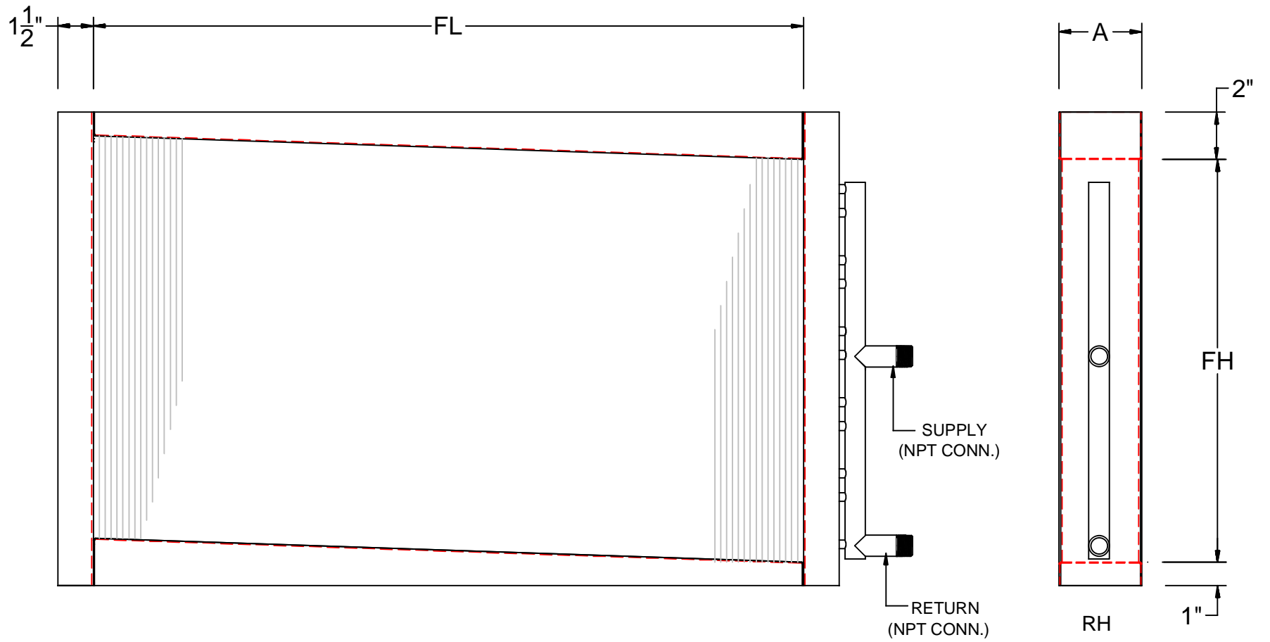
STEAM DISTRIBUTING (SAME END COIL)
